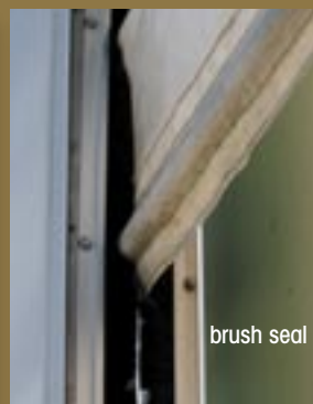
Two choices of end seals for maximum heat retention
